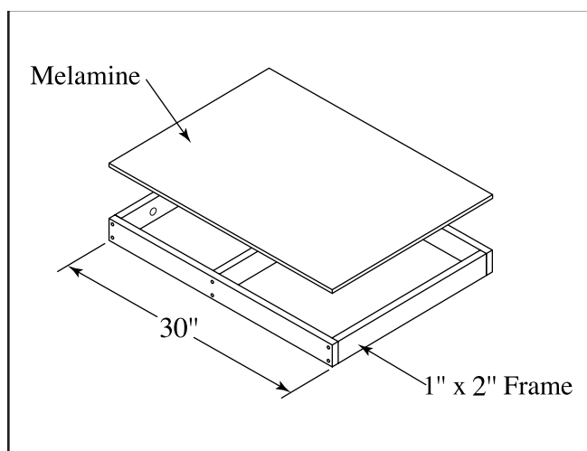
Figure 5. Extension table.
