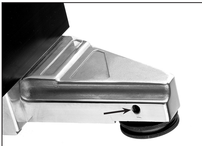
Figure 20. Loosen setscrew.
