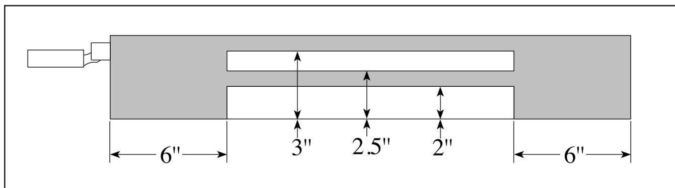
Figure 27. Side view of the fence. Do not drill in the shaded area for attaching wood facing.
