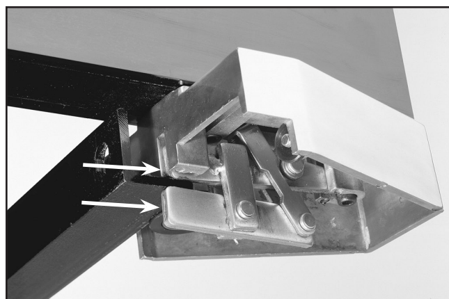
Figure 8. Jaw position.
