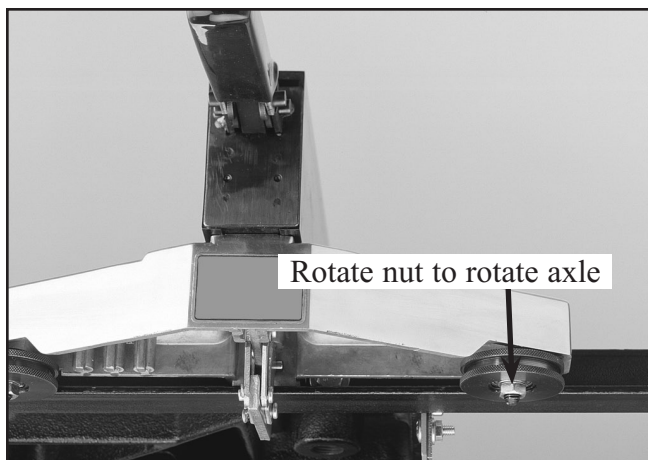
Figure 19. Adjusting the right roller axle.
