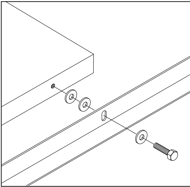
Figure 4. Mounting the rear rail.
