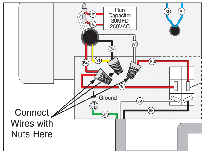
Figure 5. Model G1163/G1163P rewired to 240V.
