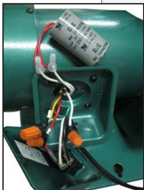
Figure 22. 240V junction box.
