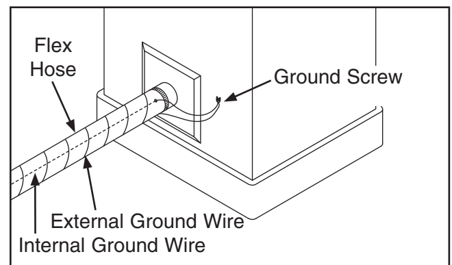
Figure 13. Flex-hose grounded to machine.
