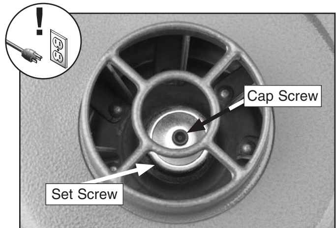
Figure 20. Impeller screw locations.
