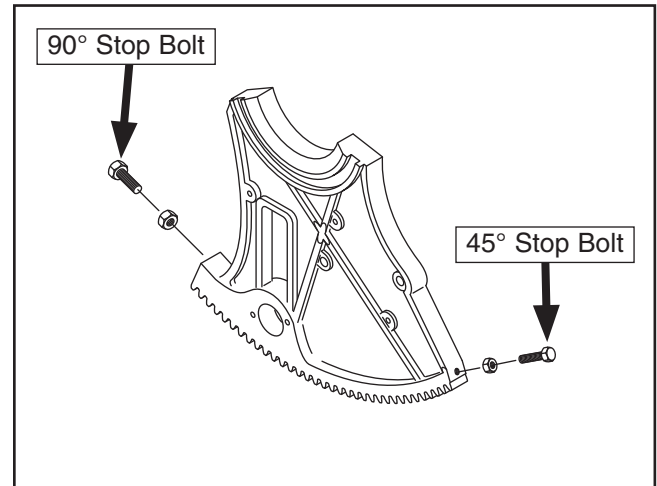
Figure 74. Geared trunnion.
