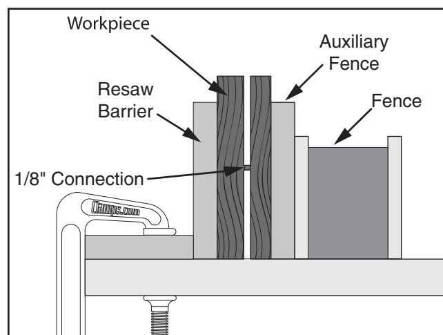
Figure 56. Ideal completed resaw cut.
