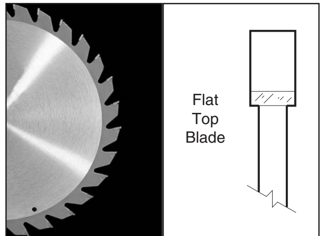
Figure 37. Ripping blade.
