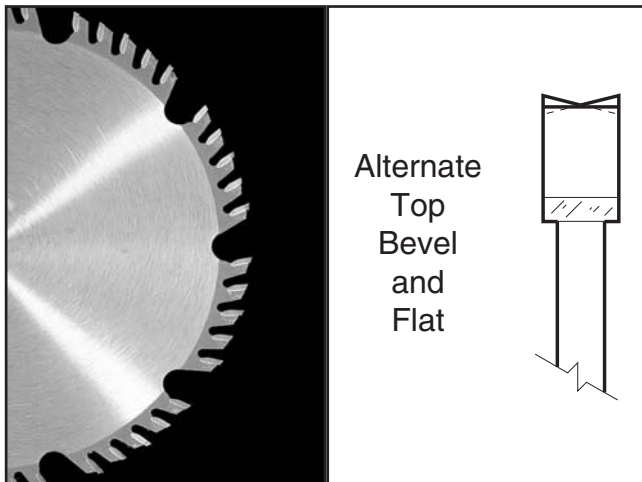
Figure 39. Combination blade.
