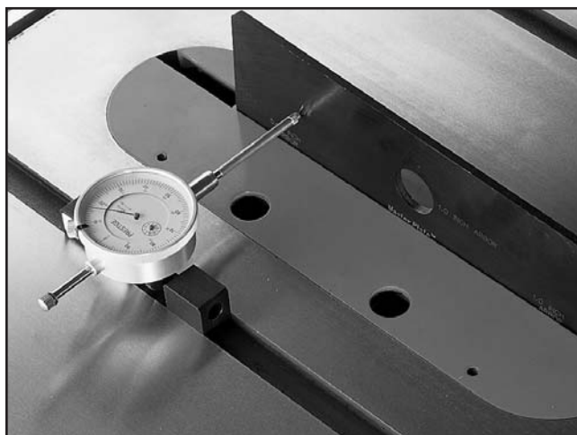
Figure 73. Superbar™ and Master Plate.
