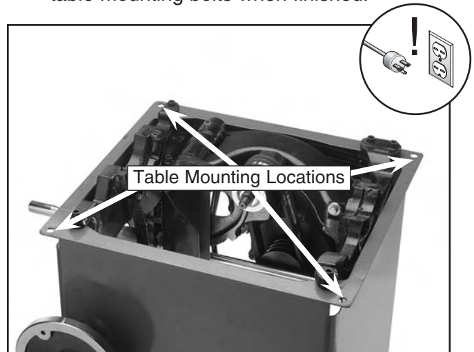
Figure 76. Table mounting bolt holes.
