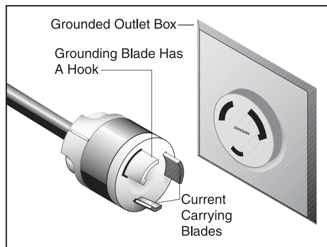
Figure 2. NEMA L6-30 plug and receptacle.
