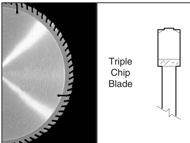
Figure 40. Laminate blade.
