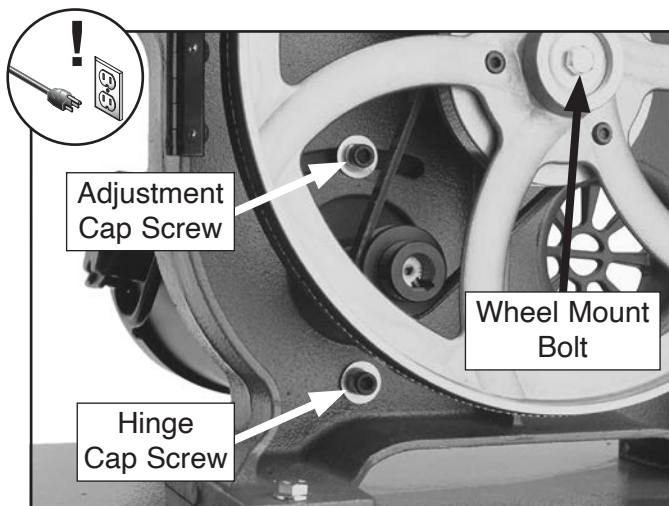
Figure 55. Locations of the wheel mount bolt, and motor adjustment and hinge cap screws.
