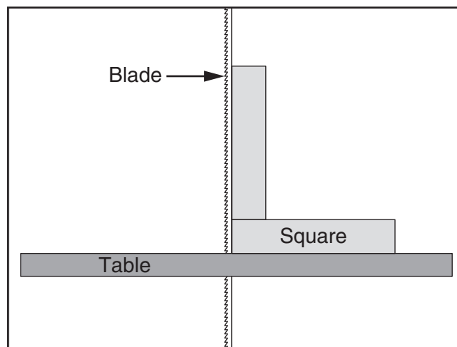
Figure 56. Checking the table to be perpendicular to the back of the blade.
