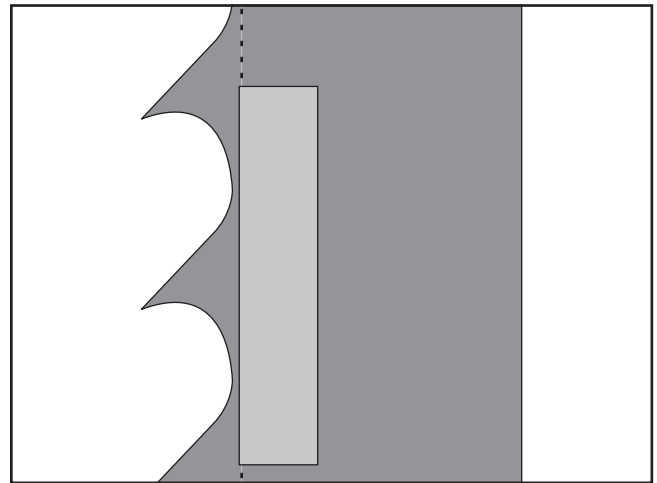
Figure 32. The blade guide bearings should be positioned just behind the blade gullets.
