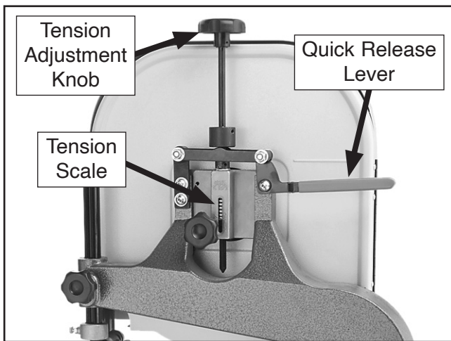
Figure 26. Blade tension controls.
