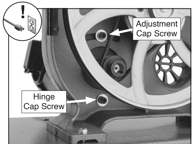
Figure 54. Locations of the motor adjustment and hinge cap screws.
