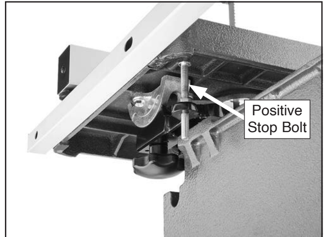
Figure 34. Positive stop bolt set at 90° (viewed from behind the table).
