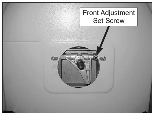
Figure 60. Front lateral adjustment set screw (viewed with the upper wheel removed).
