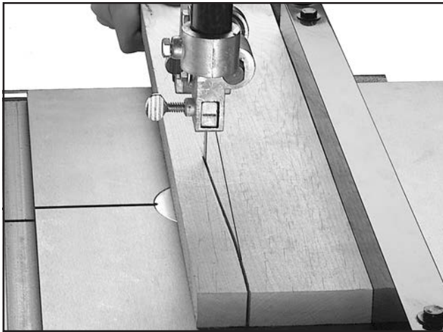
Figure 62. Example of blade lead.
