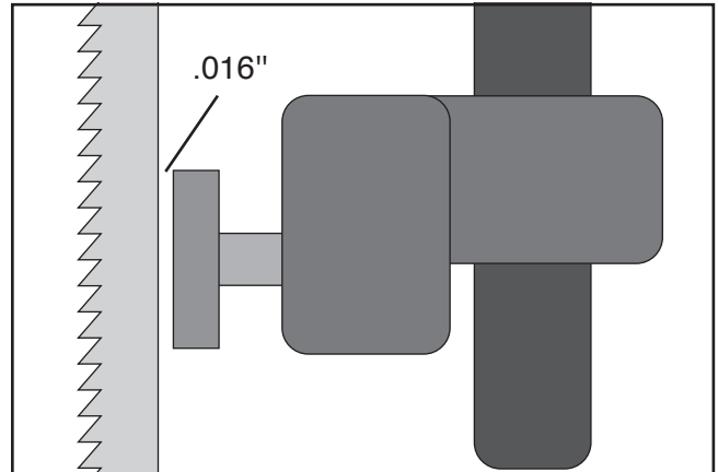
Figure 29. The face of the support blade must be approximately 0.016" behind the blade.
