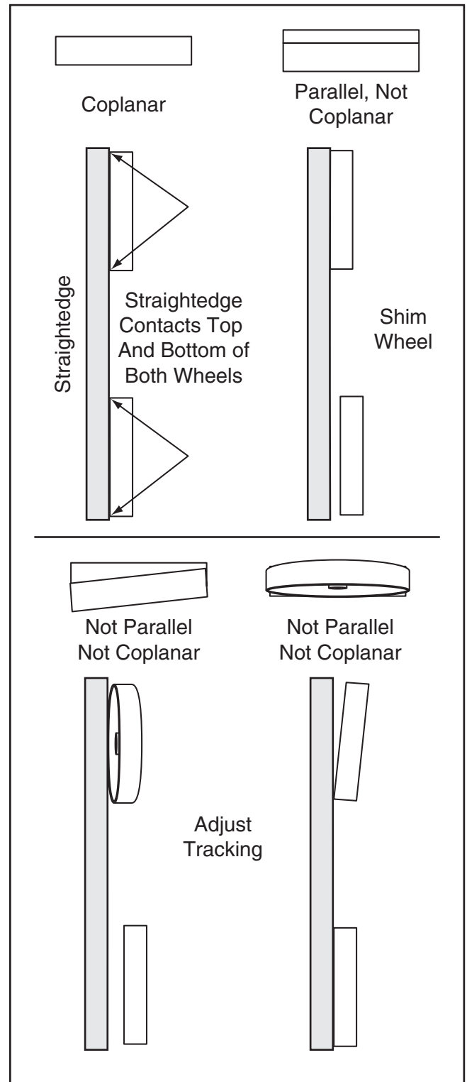
Figure 58. Wheel alignment illustration.
