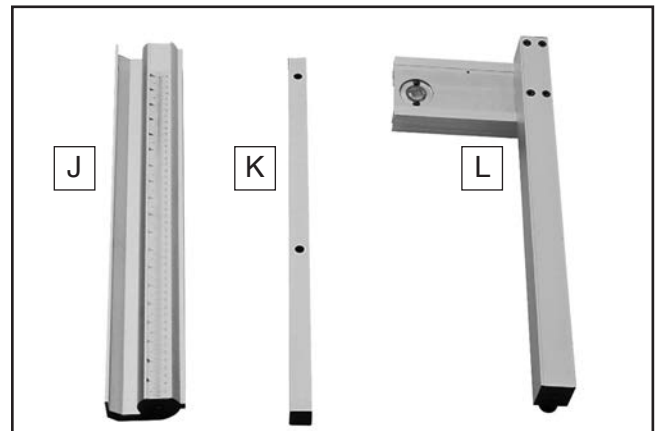
Figure 5. Fence components.
