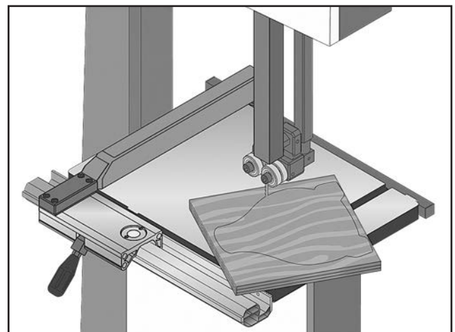
Figure 49. Example of a stacked cut setup.
