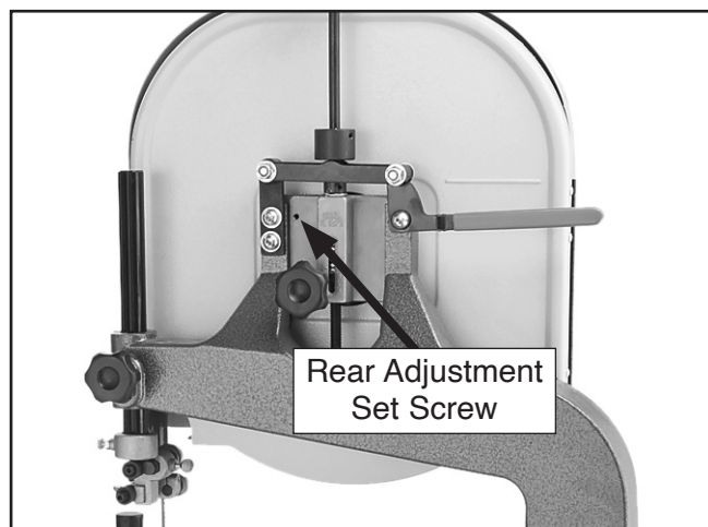
Figure 61. Rear lateral adjustment set screw.
