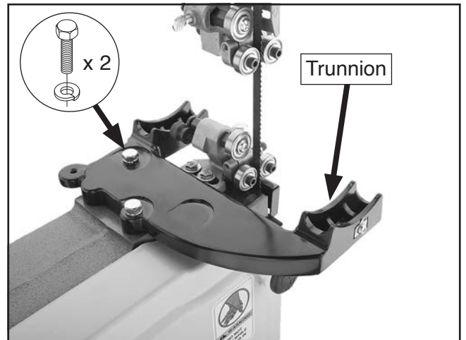
Figure 14. Trunnion installed.
