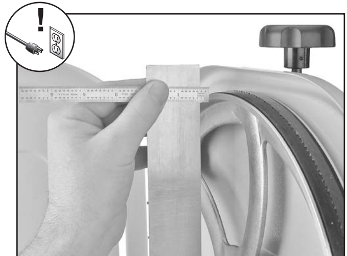
Figure 59. Measuring the distance to shim the wheel to be coplanar.
