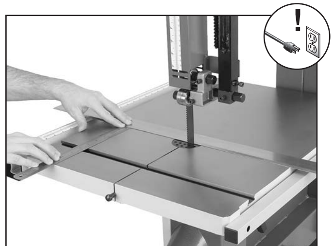
Figure 37. Measuring for table-to-blade parallelism.
