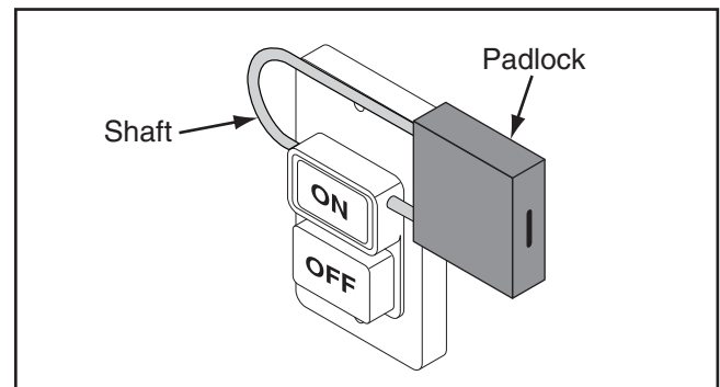
Figure 25. Switch disabling padlock inserted into ON button.
