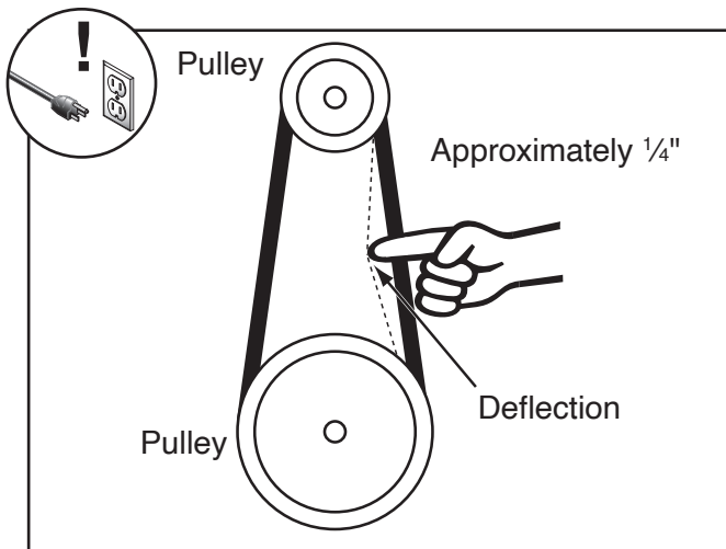
Figure 53. Checking the V-belt tension.
