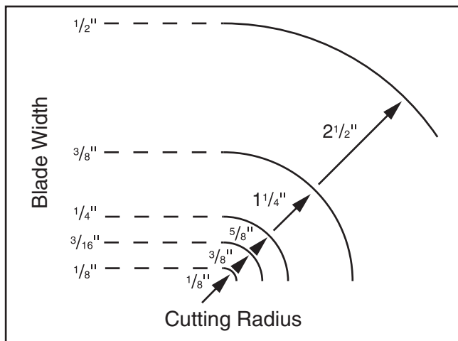
Figure 44. Recommended cutting radius per blade width.
