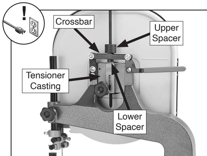
Figure 63. Locations of spacers and tensioner crossbar.
