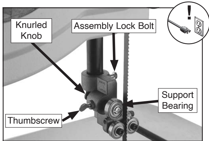
Figure 27. Support bearing controls.
