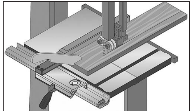
Figure 46. Example of a ripping operation.
