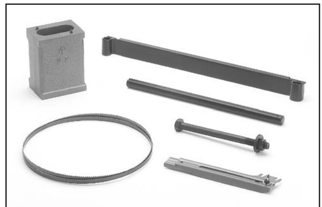
Figure 51. H3051 Extension Block Kit.
