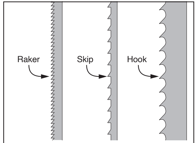
Figure 45. Main blade tooth styles.
