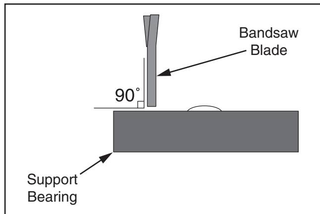
Figure 28. The face of the support bearing must be perpendicular (90°) to the blade.
