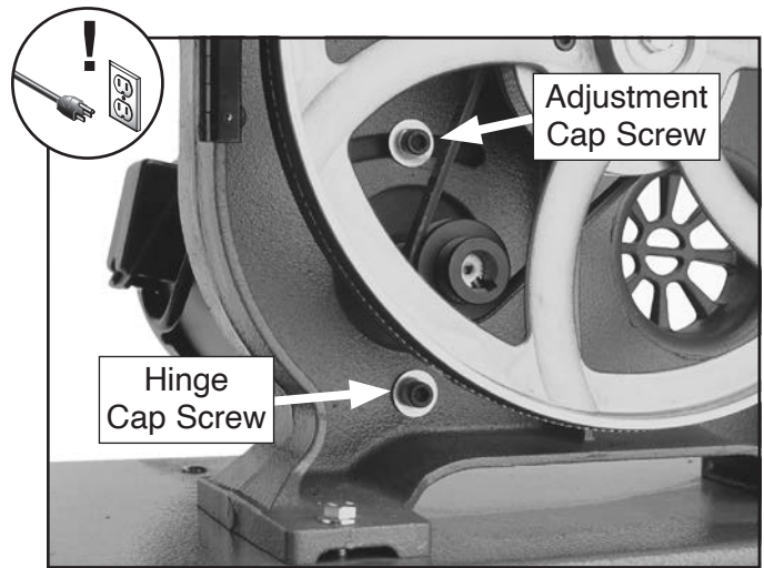
Figure 42. Locations of the motor adjustment and hinge cap screws.
