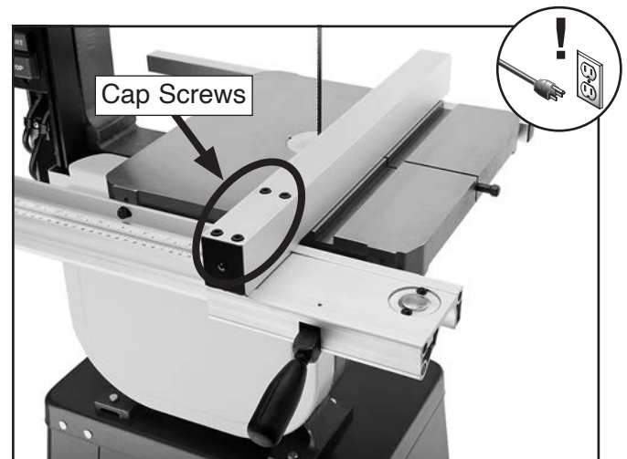
Figure 39. Location of the fence adjustment cap screws.
