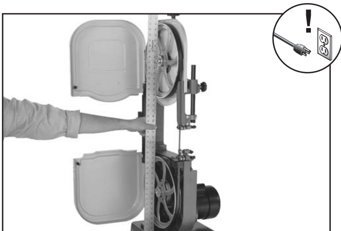
Figure 57. Checking if the wheels are coplanar.
