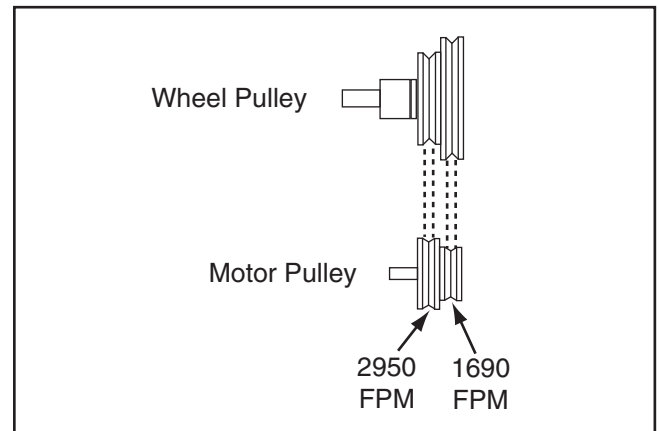
Figure 43. Drive belt position for the different speeds.
