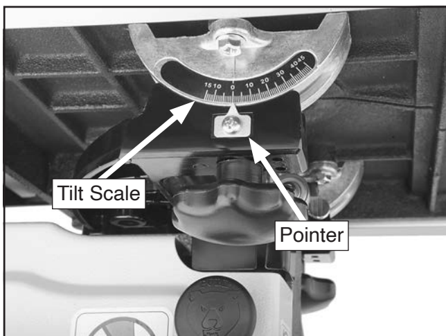
Figure 36. Location of the table tilt scale.
